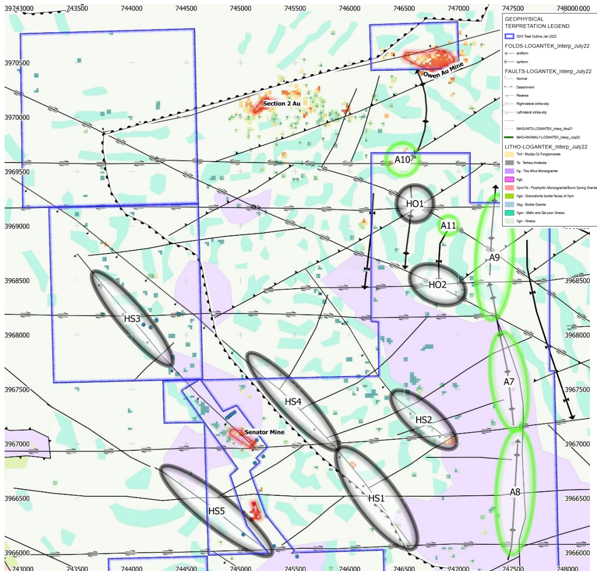
Figure 6 - Senator and Owen's Area Gold Targets
