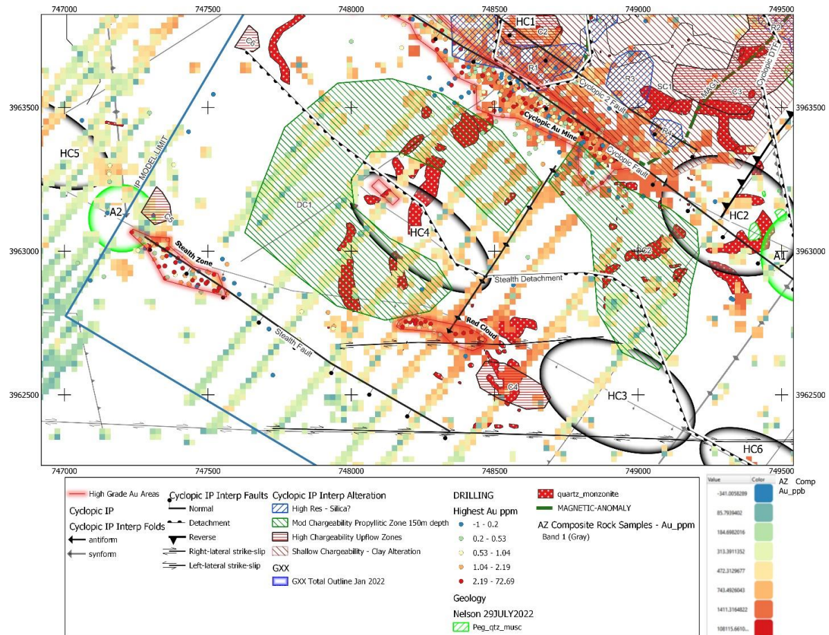
Figure 3 - Target 3 - STEALTH DTF, highlighted in yellow
