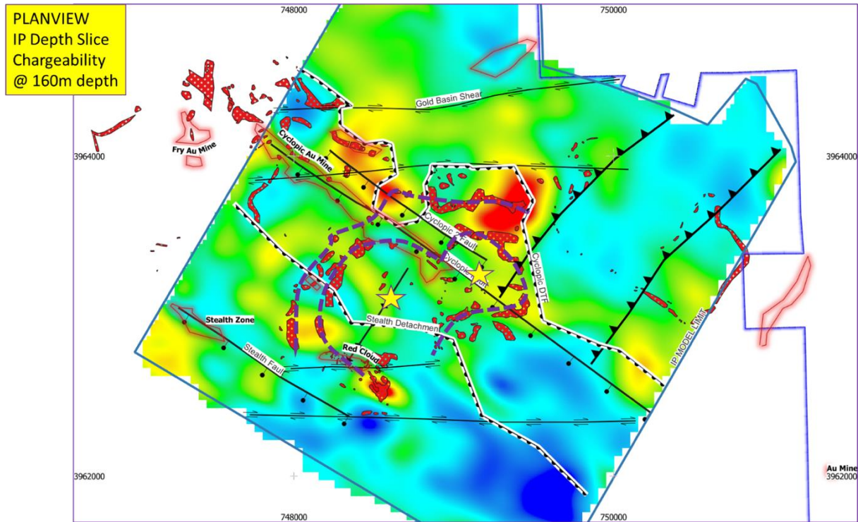
Figure 5 – Chargeability at 160m depth and Quartz Monzogranite dykes forming two concentric rings. The 2 yellow stars show the inferred centers
