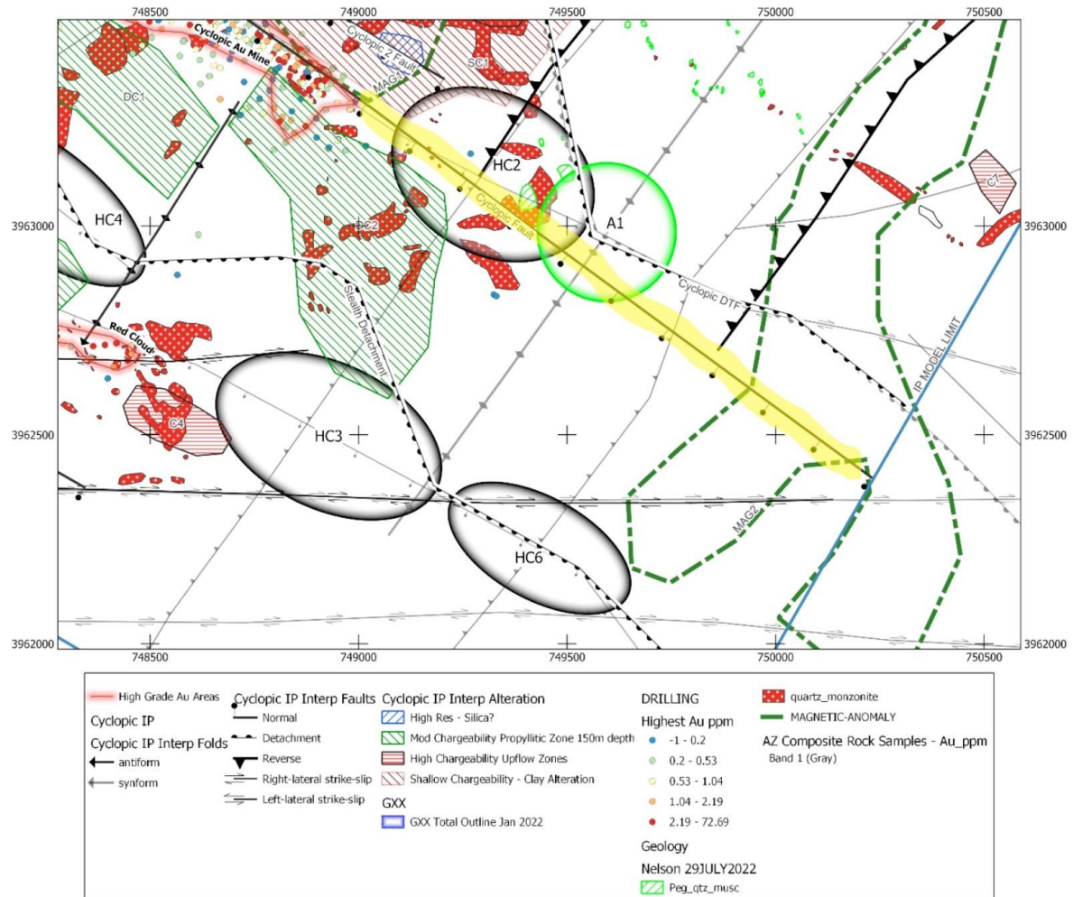
Figure 2 - Target Area 2 is the SE extension of the Cyclopic Fault in yellow
