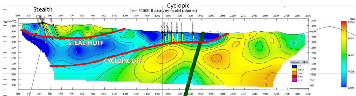
Figure 4 - Line 5200E Resistivity showing the cross-section of Stealth and Cyclopic DTF
