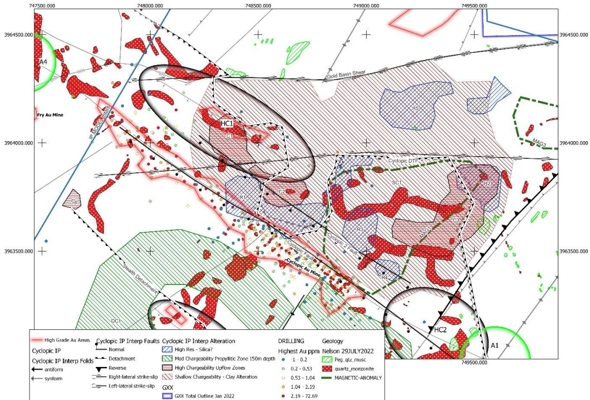
Figure 1 – Targets within the Cyclopic-Stealth area
