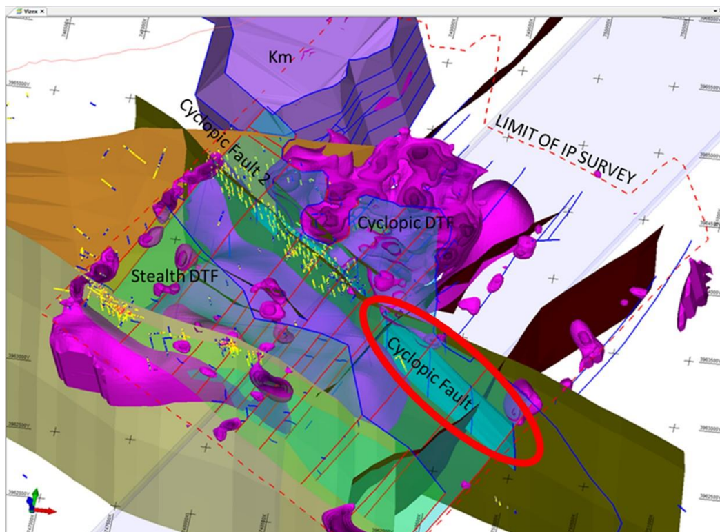
Figure 2a - Target Area 2 is the SE extension of the Cyclopic Fault in 3D
