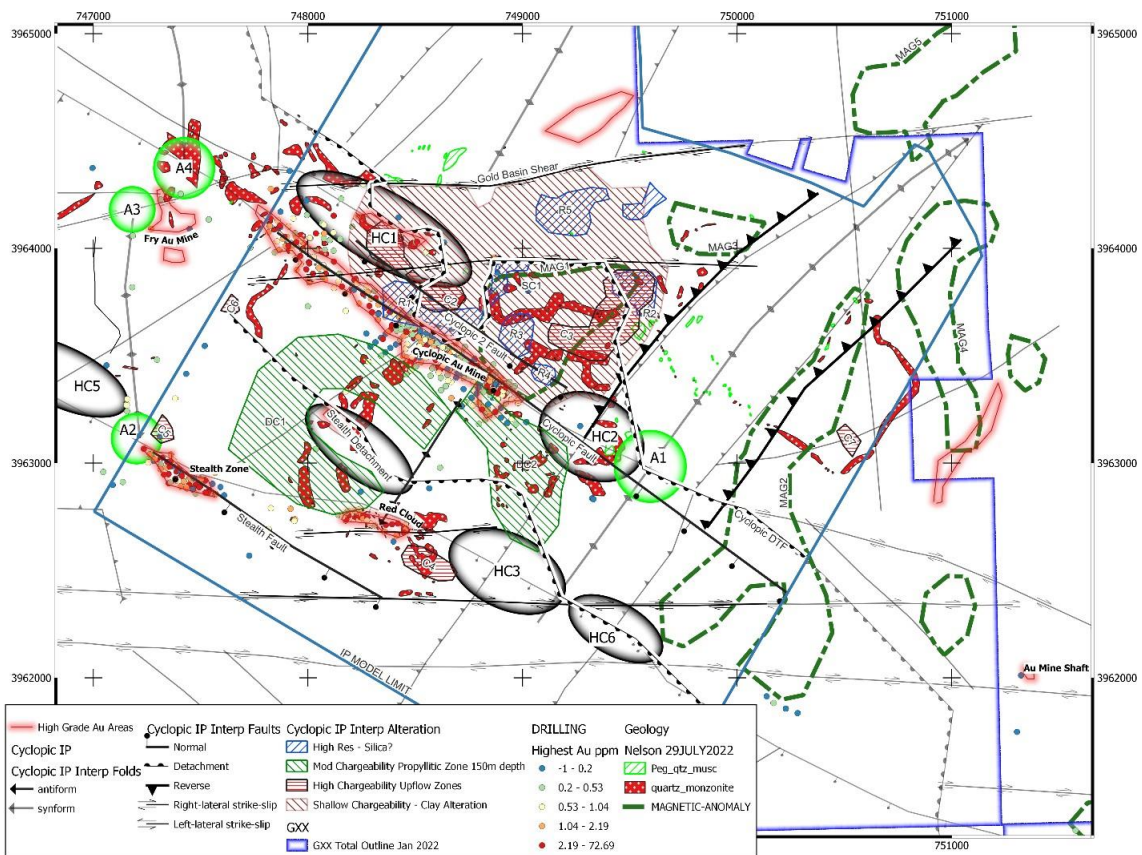
Figure 1 – Targets within the Cyclopic-Stealth area
